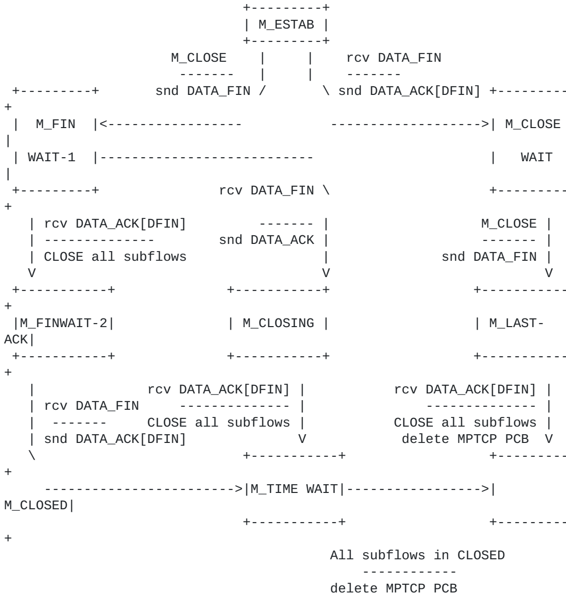
Figure 17: Finite State Machine for Connection Closure
