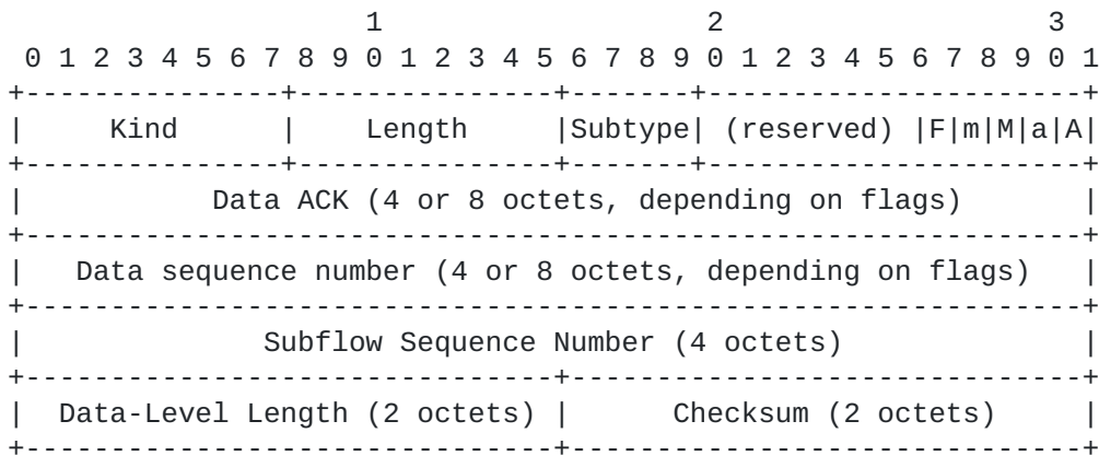
Figure 9: Data Sequence Signal (DSS) Option
