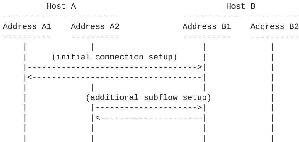
Figure 2: Example MPTCP Usage Scenario
