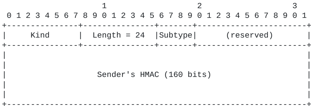
Figure 7: Join Connection (MP_JOIN) Option (for Third ACK)
