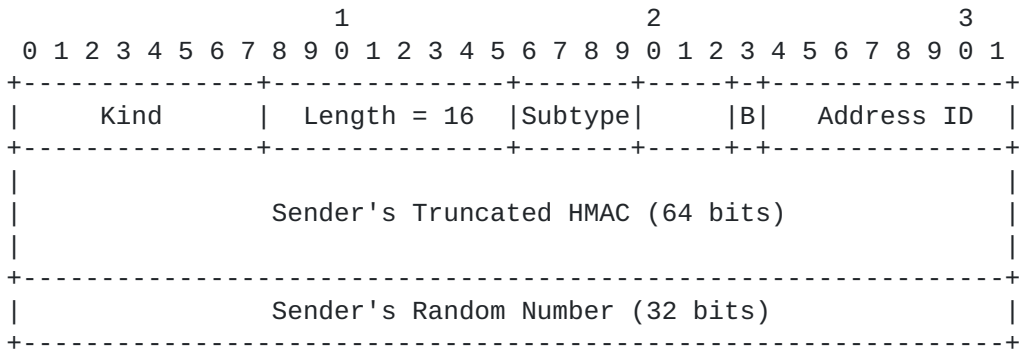
Figure 6: Join Connection (MP_JOIN) Option (for Responding SYN/ACK)
