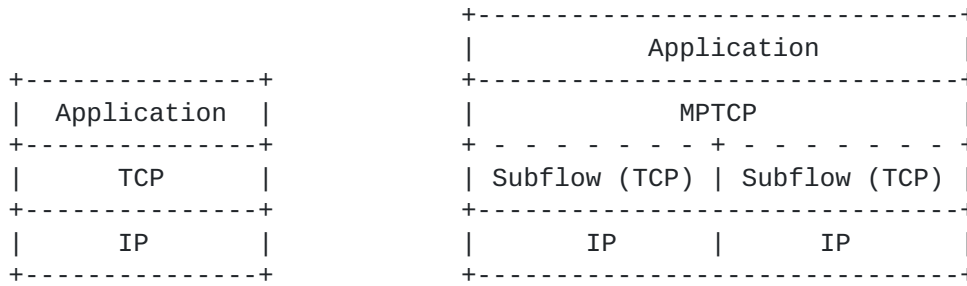
Figure 1: Comparison of Standard TCP and MPTCP Protocol Stacks
