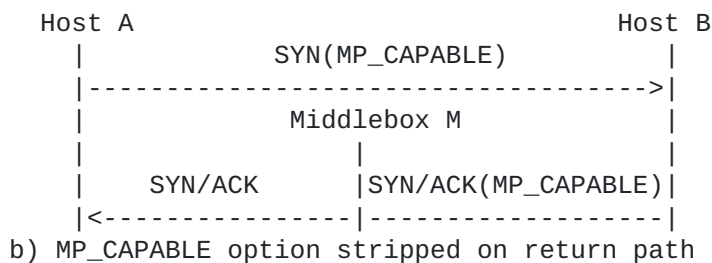
Figure 16: Connection Setup with Middleboxes that Strip Options from Packets
