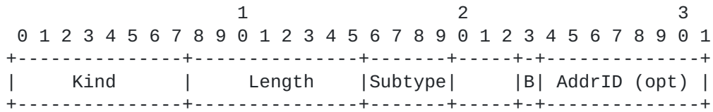
Figure 11: Change Subflow Priority (MP_PRIO) Option
