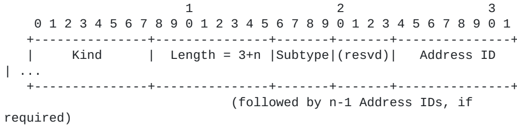
Figure 13: Remove Address (REMOVE_ADDR) Option
