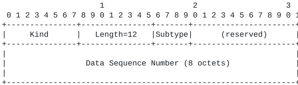
Figure 15: Fallback (MP_FAIL) Option
