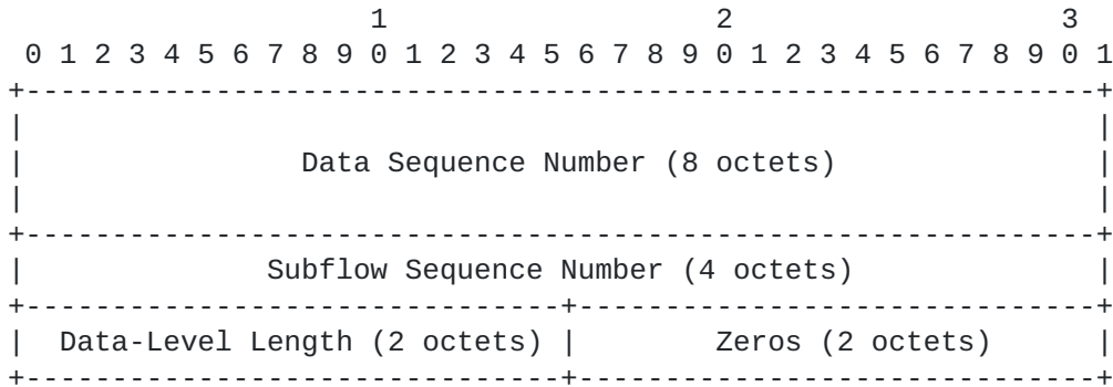
Figure 10: Pseudo-Header for DSS Checksum
