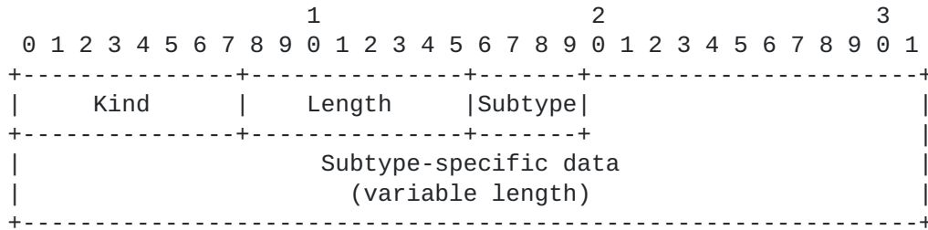
Figure 3: MPTCP Option Format
