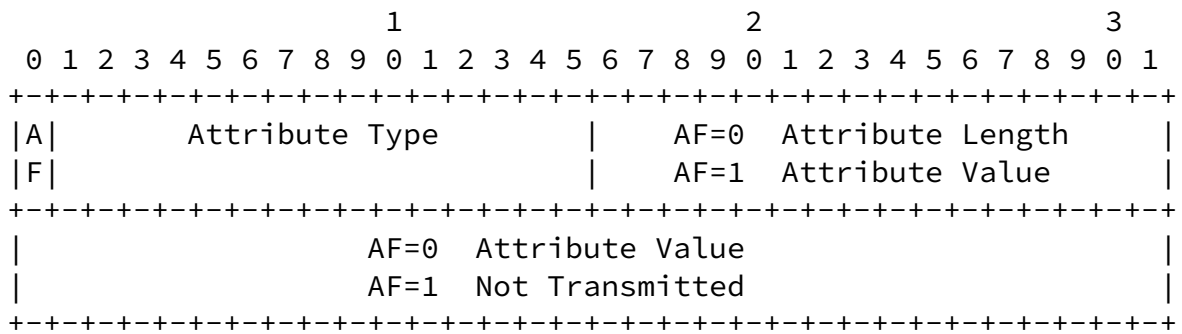
Figure 9: Data Attributes
