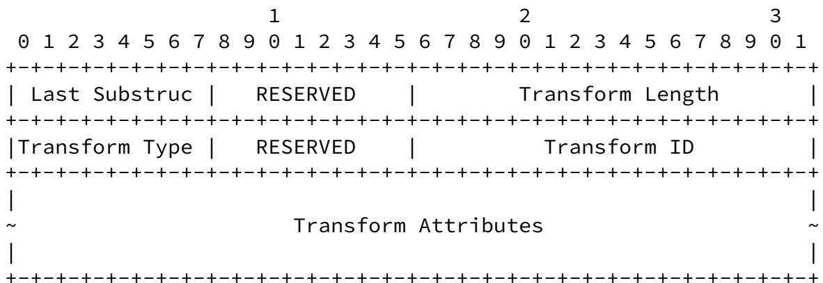
Figure 8: Transform Substructure
