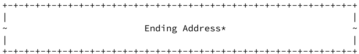
Figure 20: Traffic Selector
