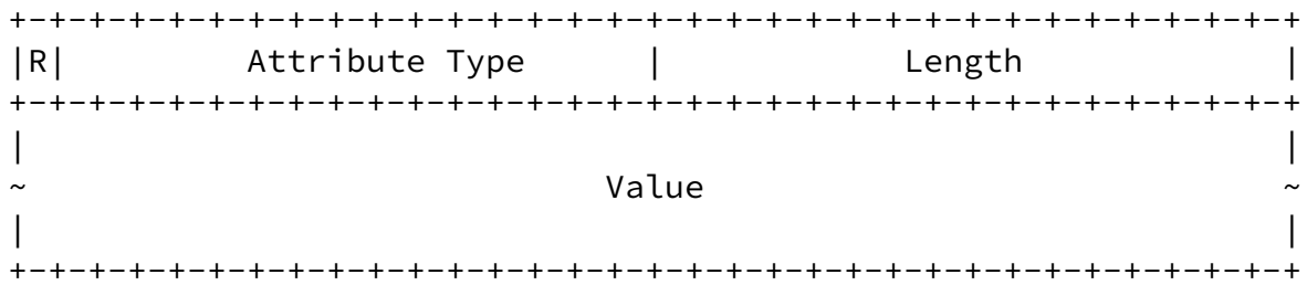
Figure 23: Configuration Attribute Format
