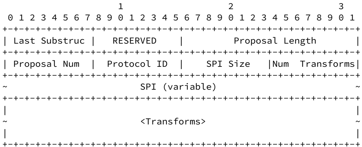
Figure 7: Proposal Substructure
