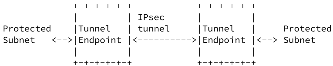
Figure 1: Security Gateway to Security Gateway Tunnel
