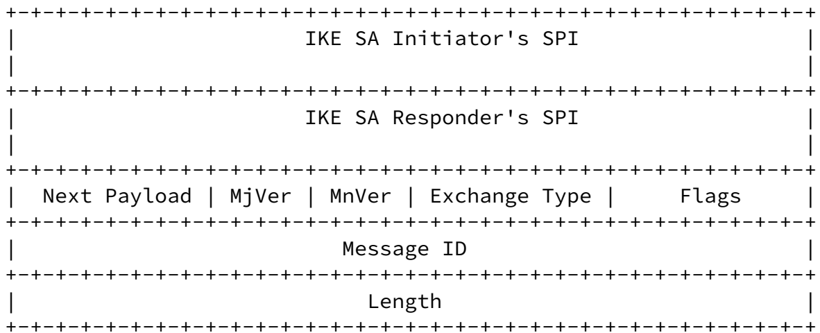
Figure 4: IKE Header Format
