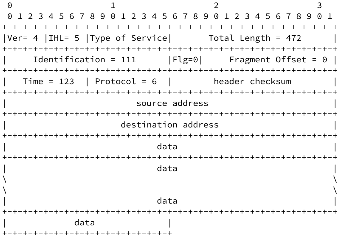
Example Internet Datagram
