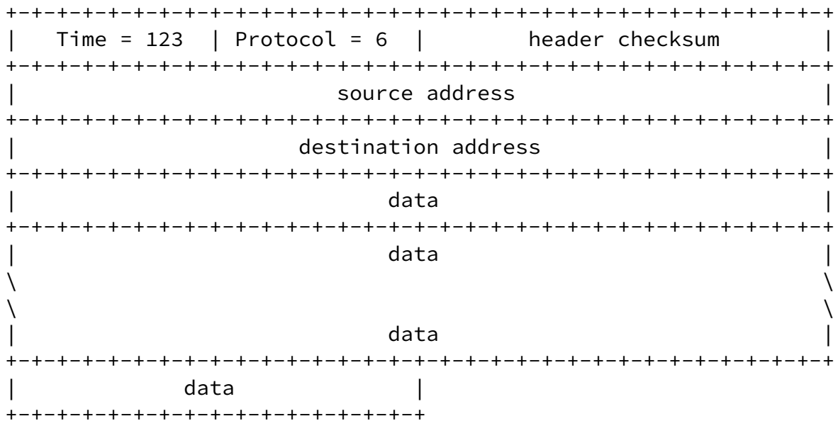
Example Internet Datagram
