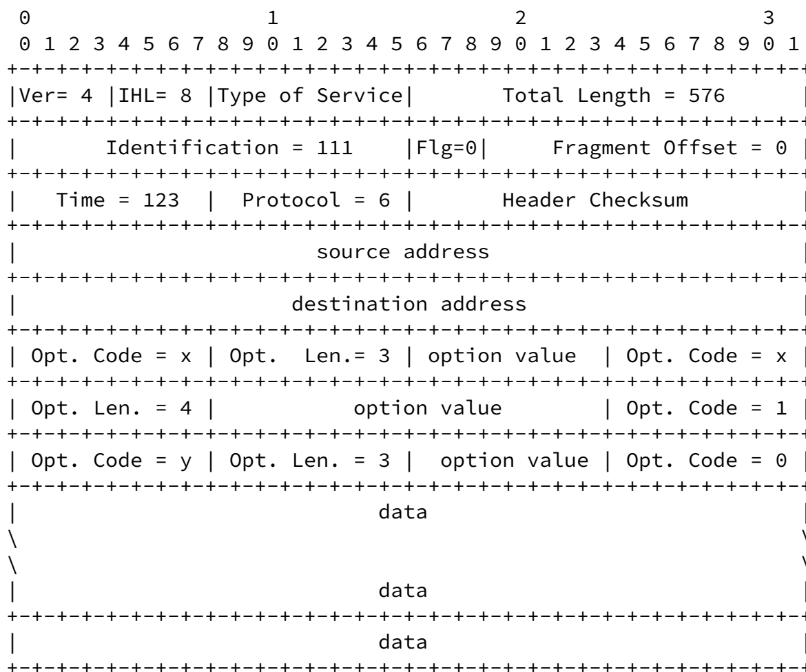
Example Internet Datagram
