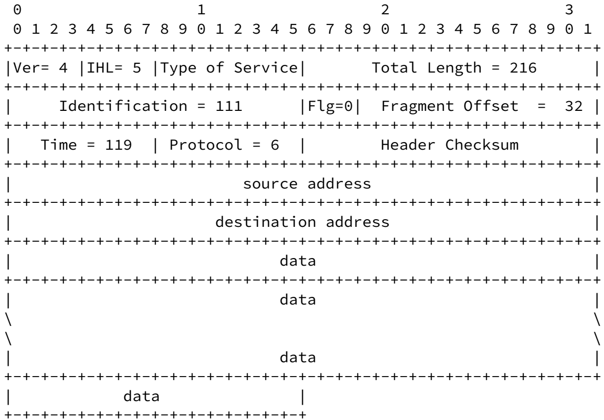
Example Internet Fragment
