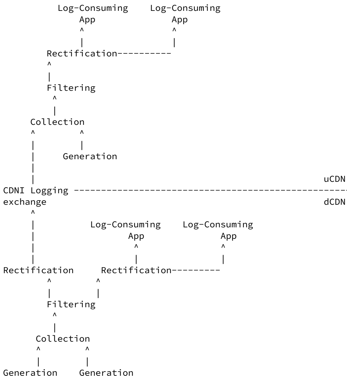
Figure 2: CDNI Logging in the Overall Logging Chain
