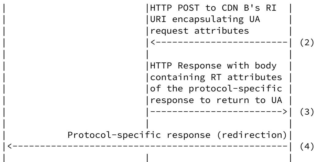
Figure 1: Generic Recursive Request Redirection Message Flow
