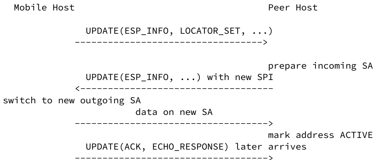
Figure 7: Address Activation via Use of a New SA
