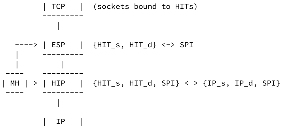
Figure 2: Architecture for HIP Host Mobility and Multihoming
