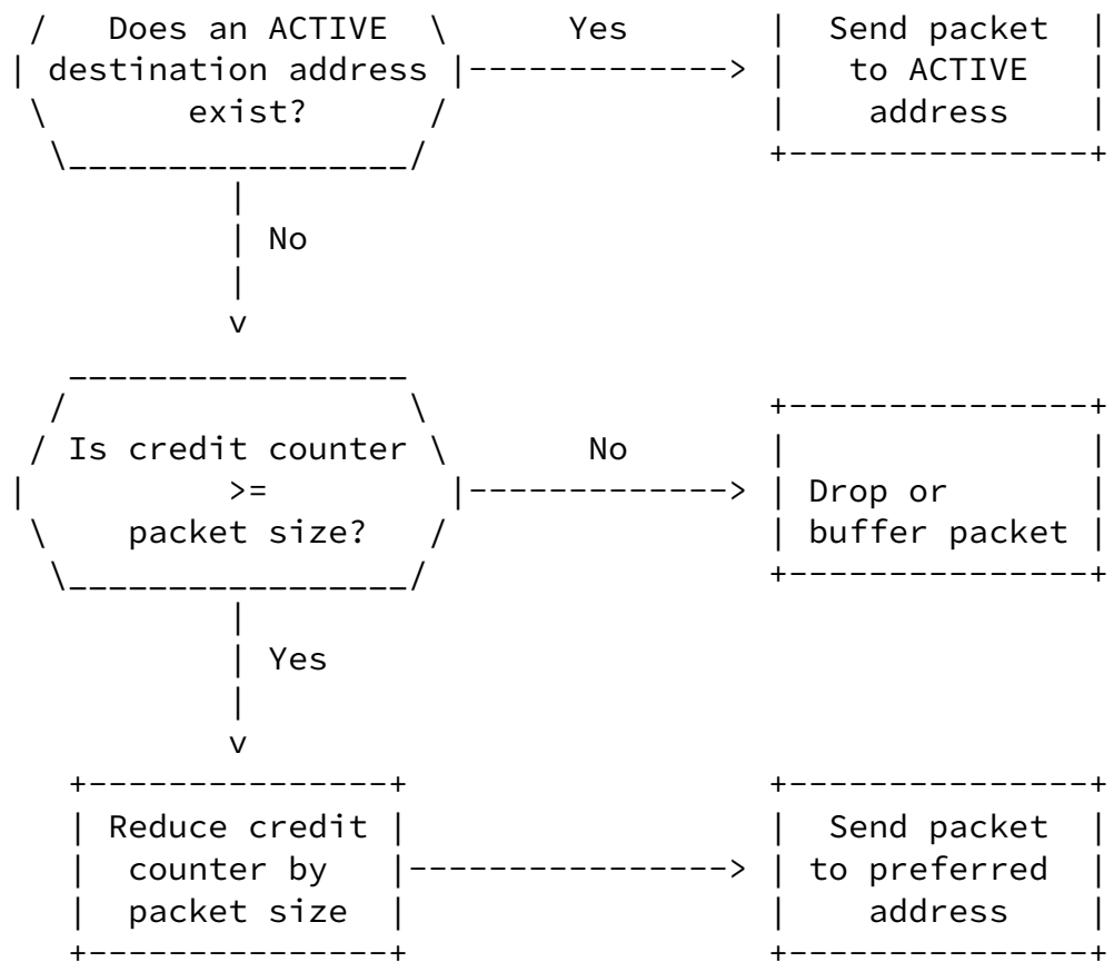
Figure 9: Sending Packets with Credit-Based Authorization
