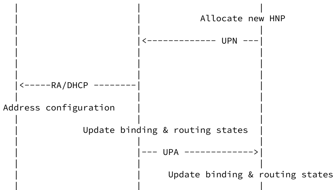
Figure 1: Signaling Call Flow for HNP Renumbering
