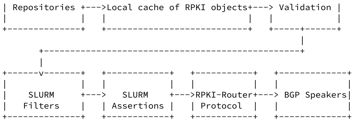
Figure 1: SLURM's Position in the RP Stack
