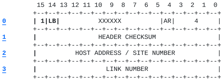
Figure 28 . RESTART COMPLETE
