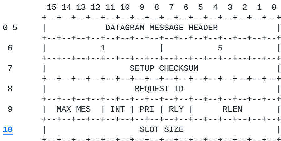
Figure 10 . CREATE STREAM REQUEST
