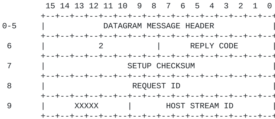
Figure 11 . CREATE STREAM REPLY
