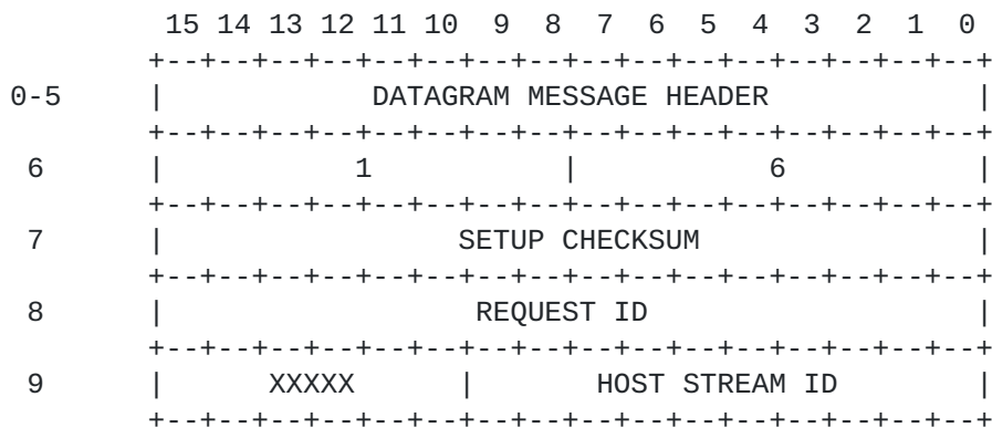
Figure 14 . DELETE STREAM REQUEST
