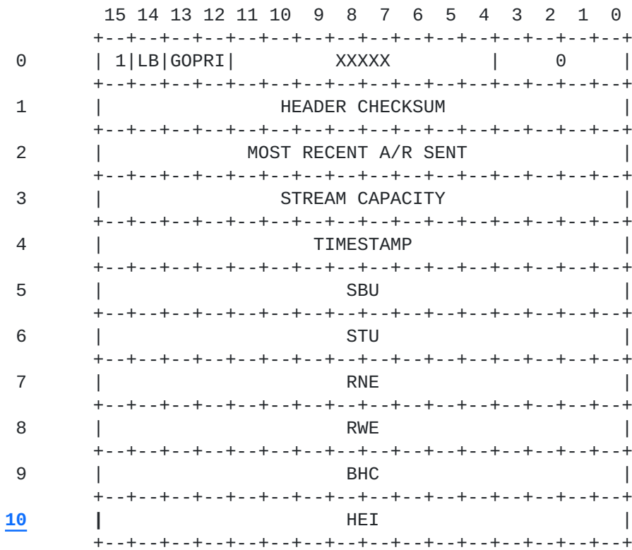
Figure 25 . STATUS MESSAGE
