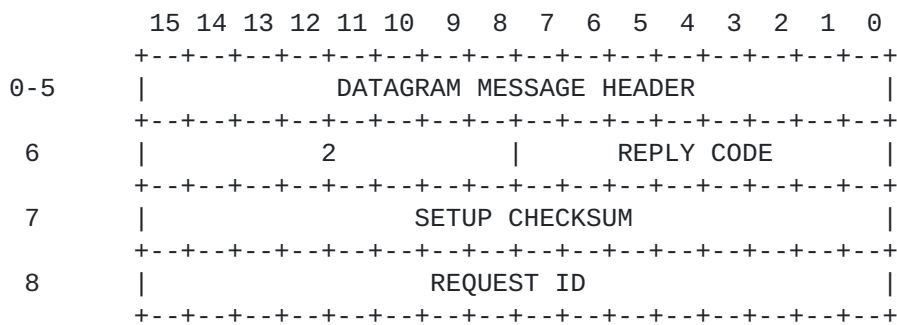
Figure 13 . CHANGE STREAM PARAMETERS REPLY
