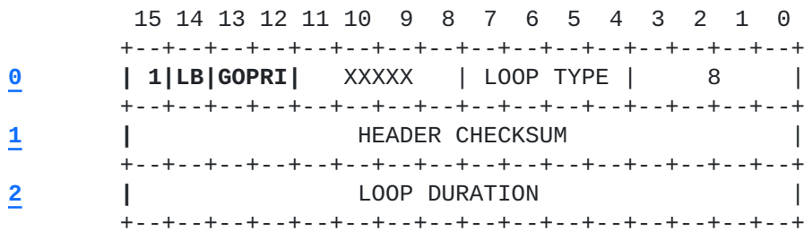
Figure 29 . LOOPBACK REQUEST
