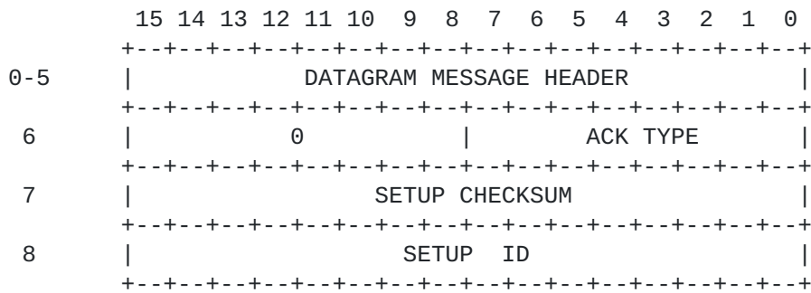
Figure 8 . SETUP ACKNOWLEDGMENT
