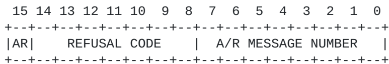
Figure 3 . ACCEPTANCE/REFUSAL WORD
