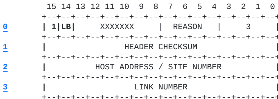
Figure 27 . RESTART REQUEST
