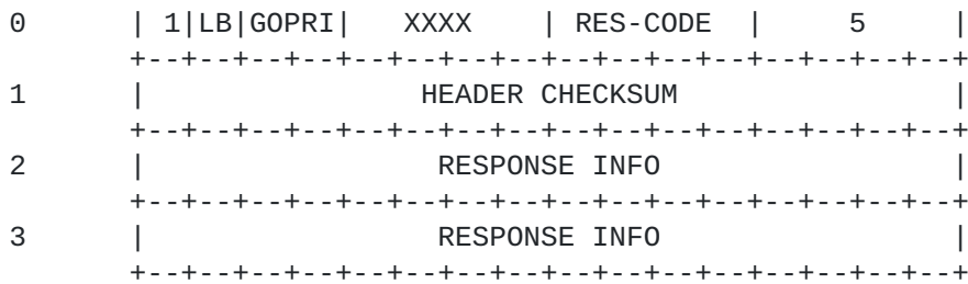
Figure 5 . UNNUMBERED RESPONSE
