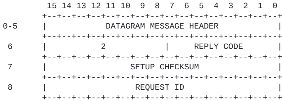
Figure 22 . LEAVE GROUP REPLY
