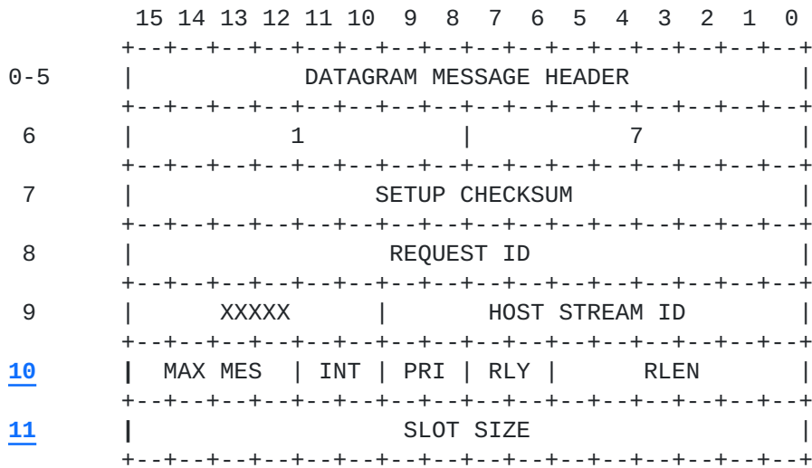
Figure 12 . CHANGE STREAM PARAMETERS REQUEST
