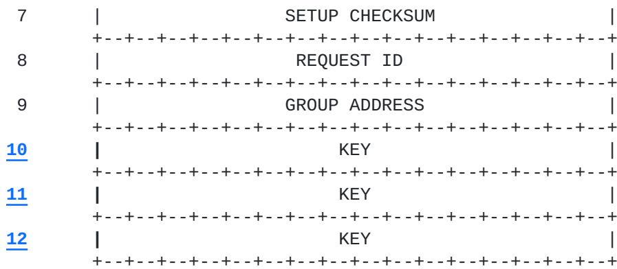
Figure 18 . CREATE GROUP REPLY
