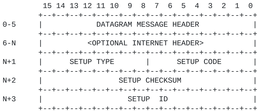
Figure 6 . SETUP MESSAGE HEADER
