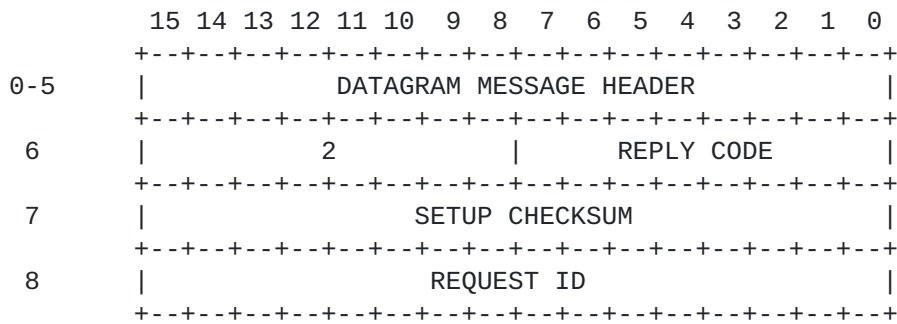
Figure 15 . DELETE STREAM REPLY
