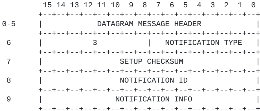
Figure 7 . NOTIFICATION MESSAGE
