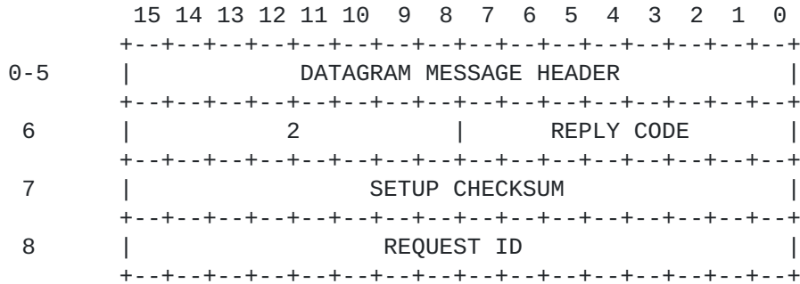
Figure 24 . DELETE GROUP REPLY
