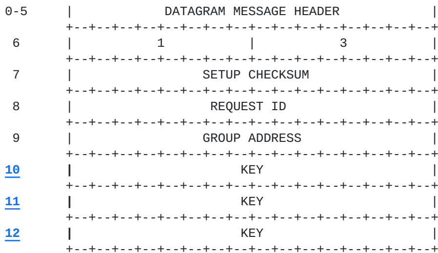
Figure 19 . JOIN GROUP REQUEST
