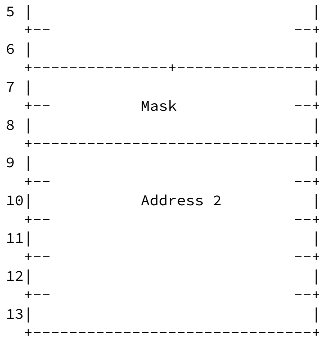
COMPARE Condition Figure 69
