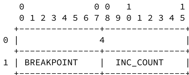
INC_COUNT Command Format Figure 73
