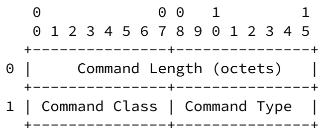
LDP Command Header Format Figure 6
