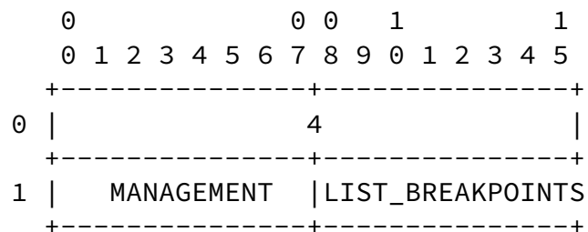
LIST_BREAKPOINTS Command Format Figure 51
