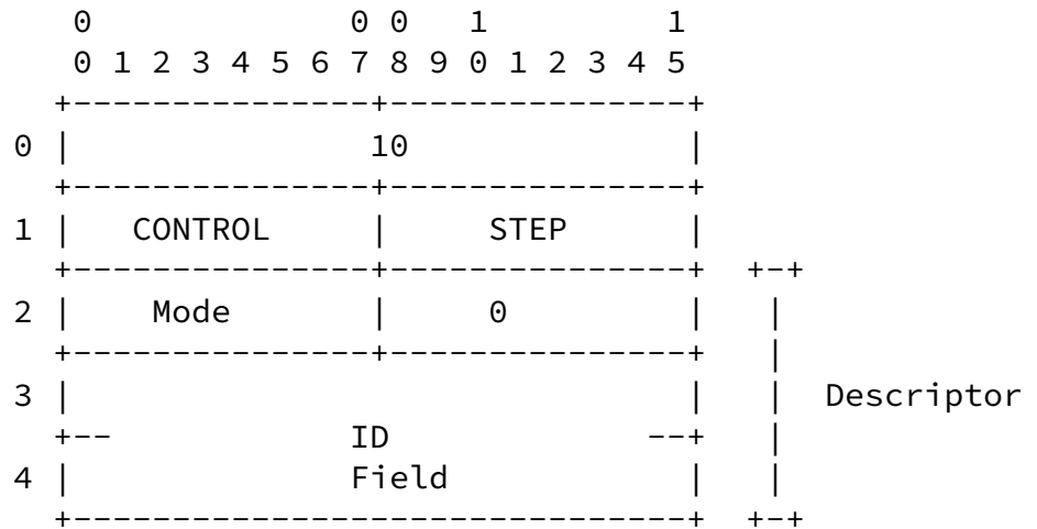
STEP Command Format Figure 38
