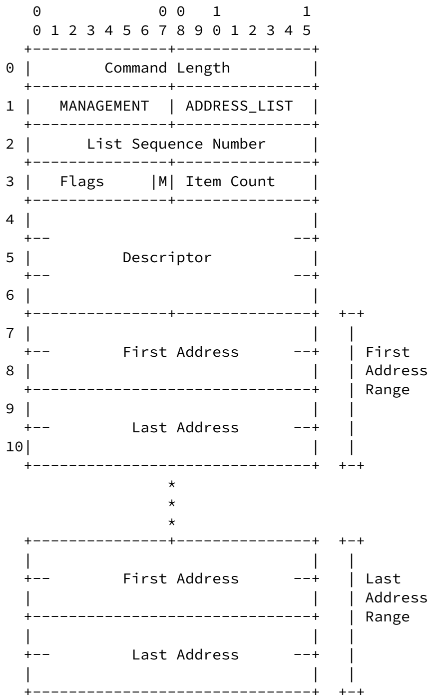
ADDRESS_LIST Reply Format Figure 50
