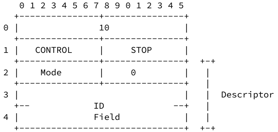
STOP Command Format Figure 36
