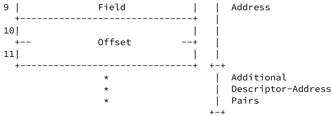
BREAKPOINT_LIST Reply Format Figure 52
