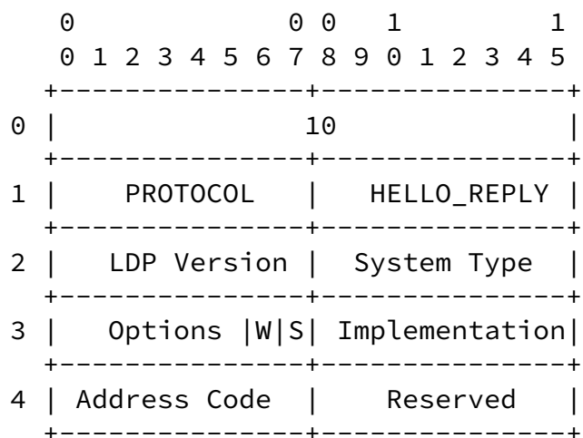
HELLO_REPLY Format Figure 14
