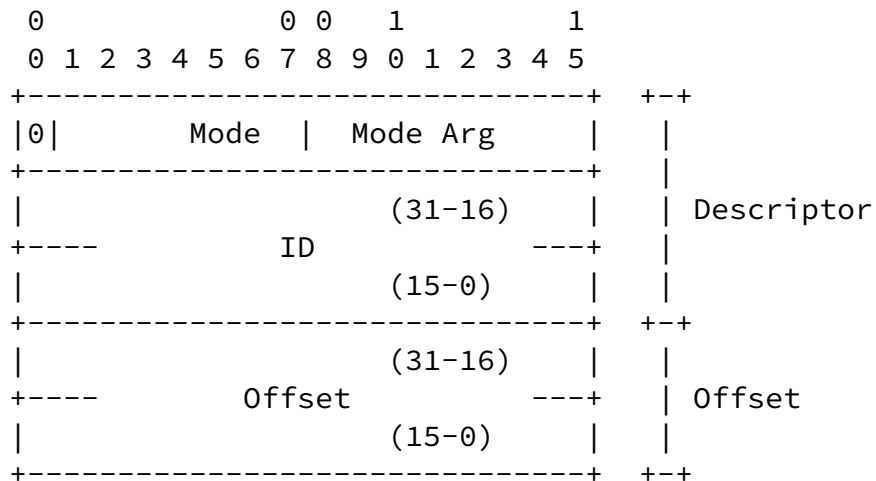
Long Format - Format bit is LONG=0
