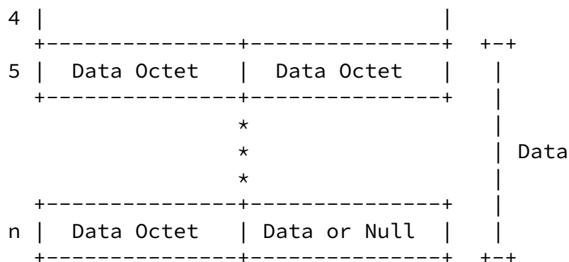
DATA Response Format Figure 28
