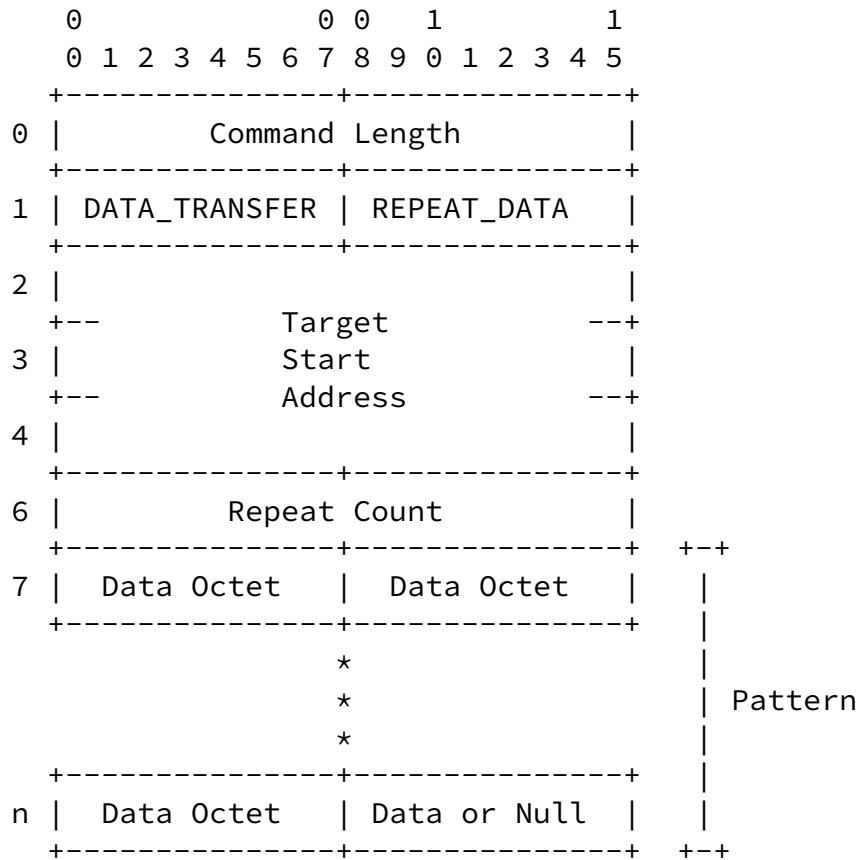
REPEAT_DATA Command Format Figure 33
