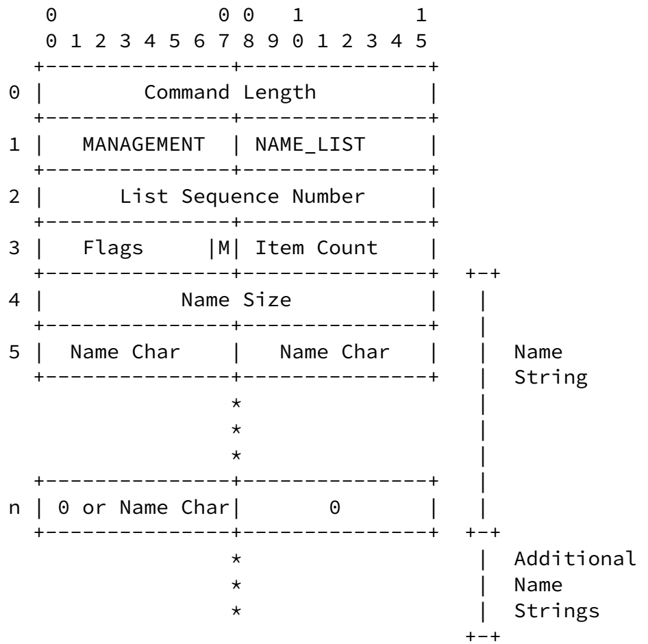
NAME_LIST Reply Format Figure 56
