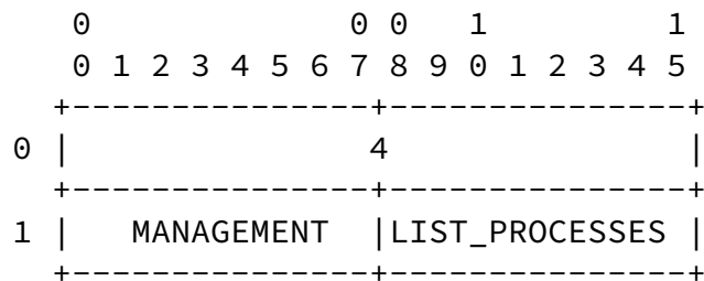
LIST_PROCESSES Command Format Figure 53
