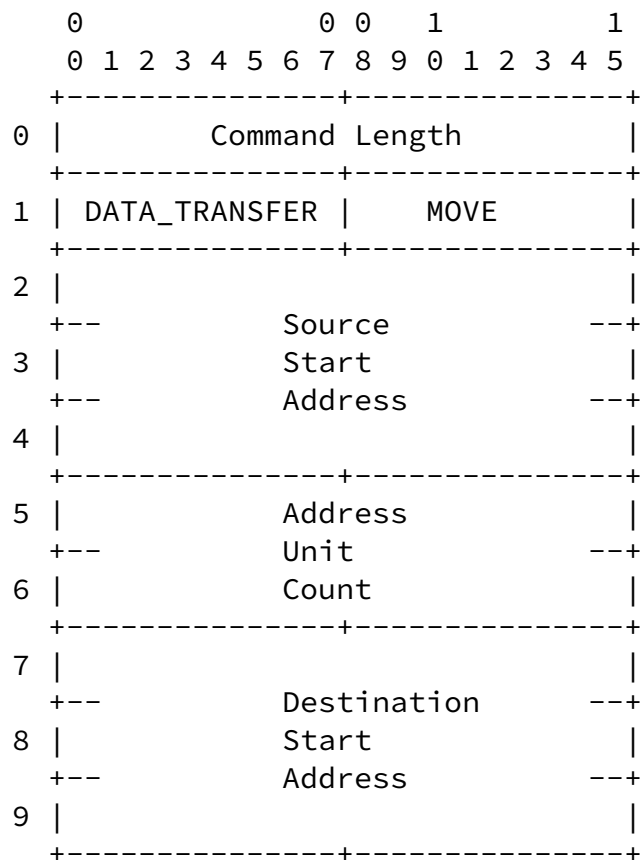
MOVE Command Format Figure 30
