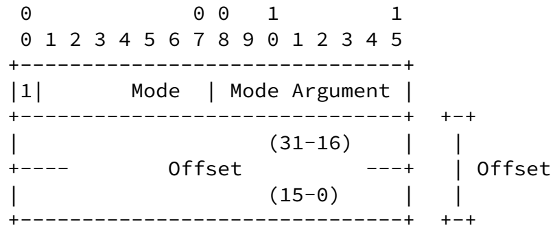
Short Address Format Figure 11
