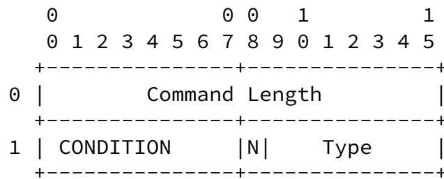
Condition Command Header Figure 66
