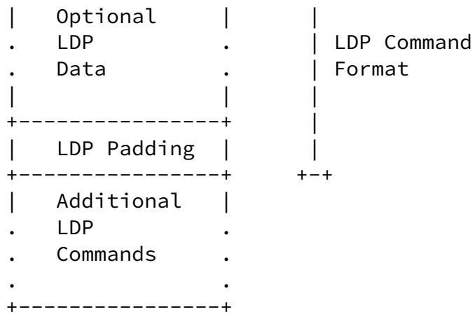
Network Packet Format Figure 5
