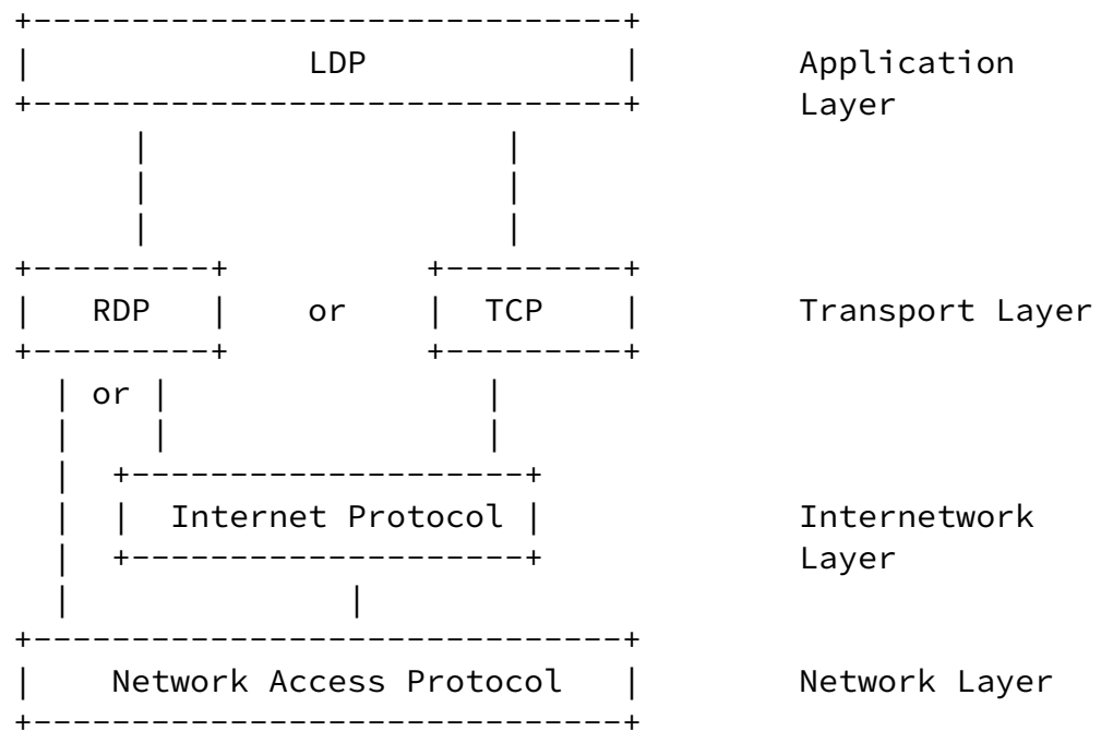
Relation to Other Protocols Figure 1
