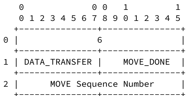
MOVE_DONE Reply Format Figure 32
