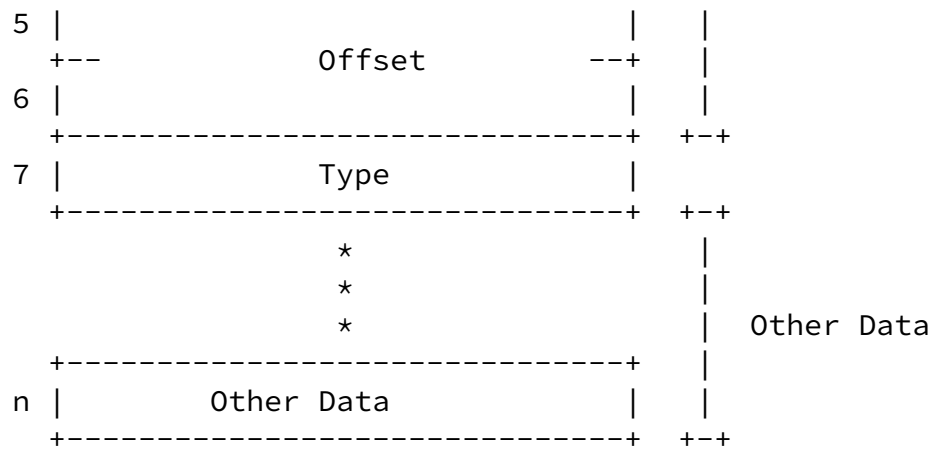
EXCEPTION Format Figure 41
