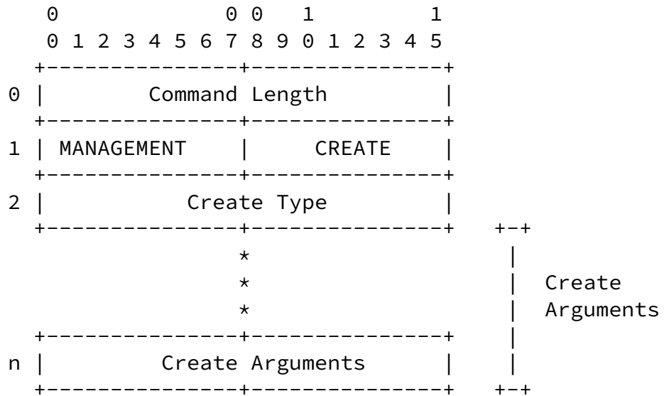
CREATE Command Format Figure 42
