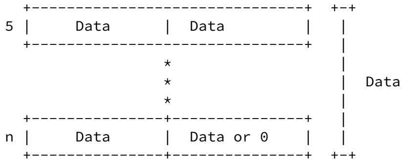
BREAKPOINT_DATA Command Format Figure 63
