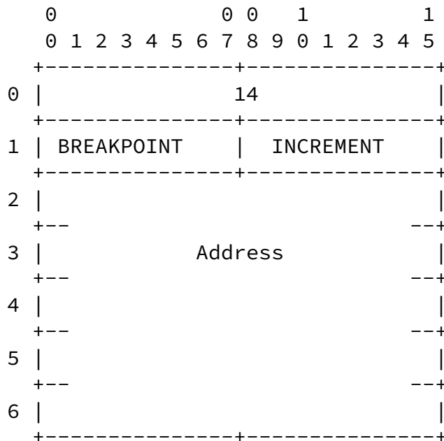
INCREMENT Command Format Figure 72
