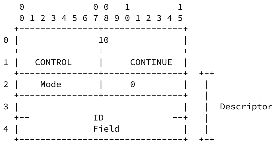
CONTINUE Command Format Figure 37
