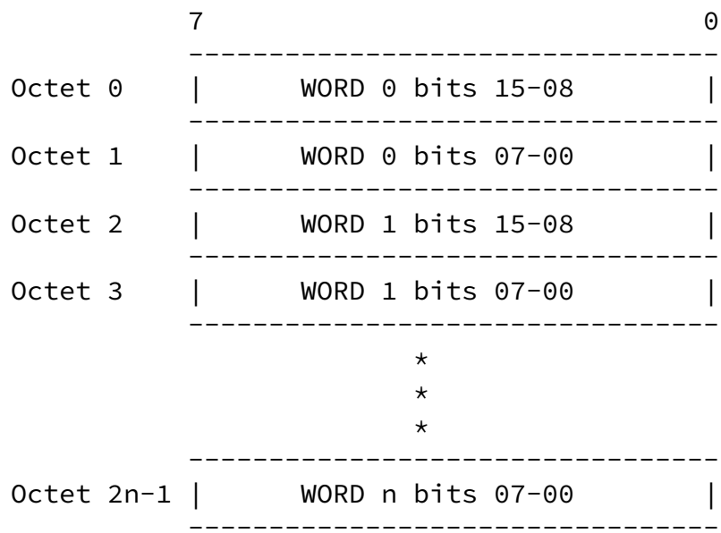
Packing of 16-bit Words Figure 3
