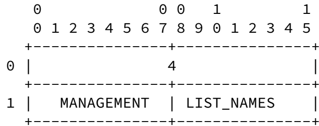
LIST_NAMES Command Format Figure 55
