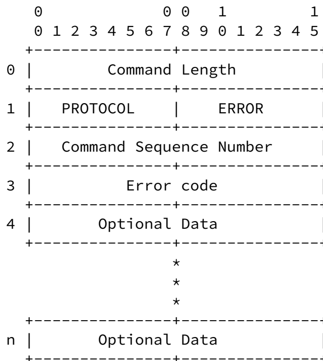
ERROR Reply Format Figure 23
