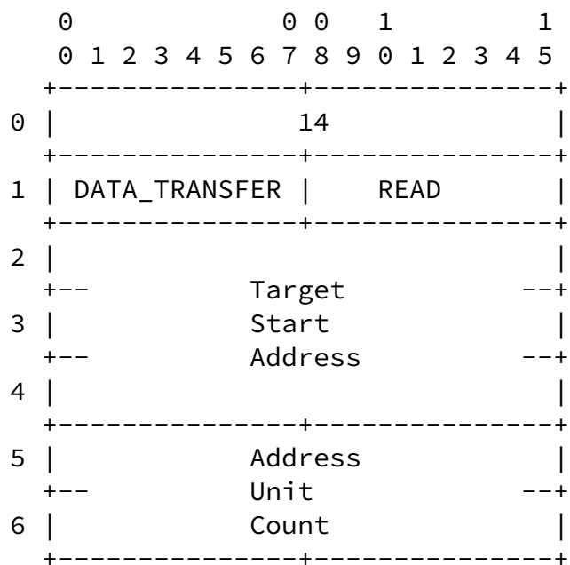
READ Command Format Figure 27
