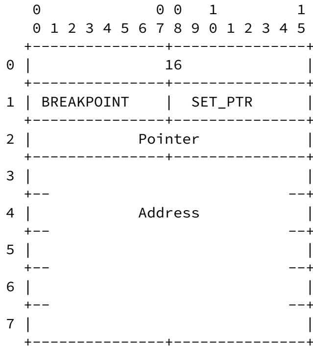
SET_PTR Command Format Figure 75
