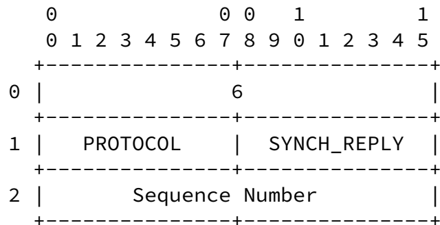
SYNCH_REPLY Format Figure 20
