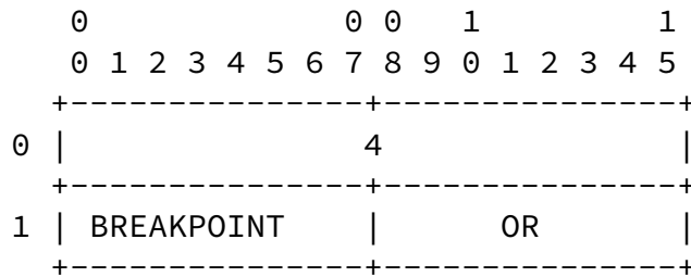
OR Command Format Figure 74
