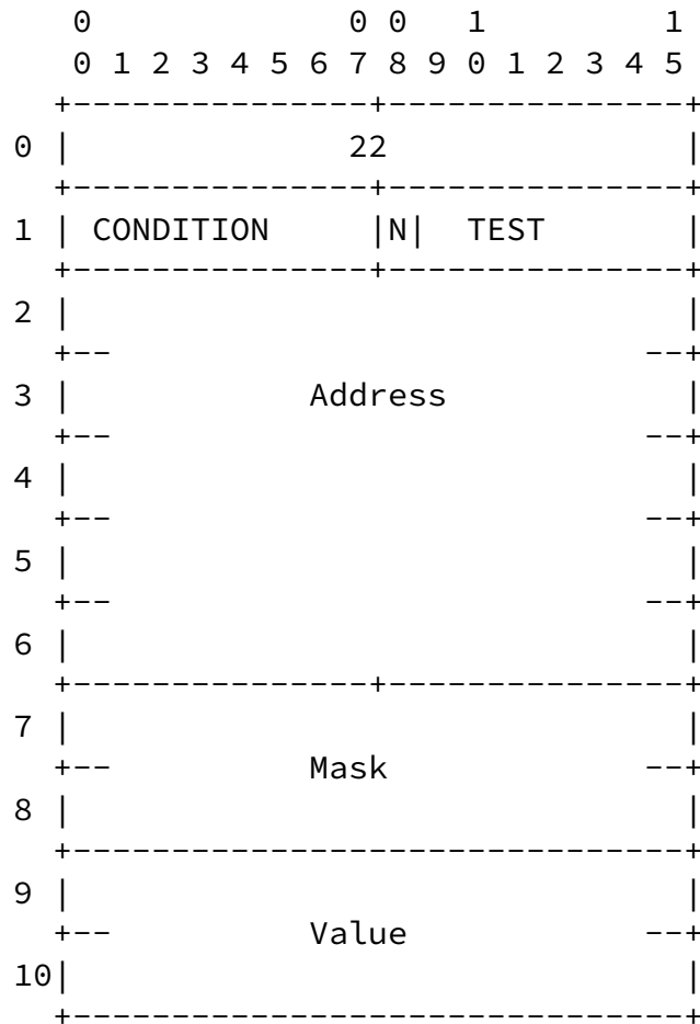
TEST Condition Figure 70
