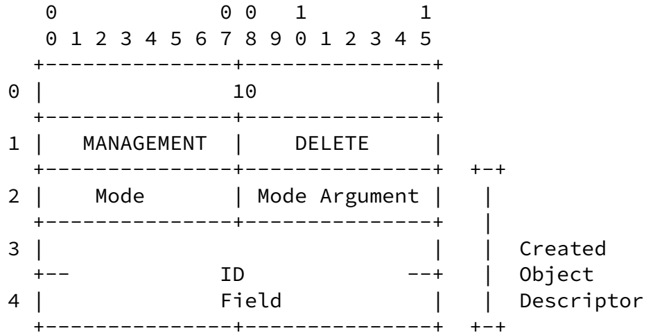
DELETE Command Format Figure 47
