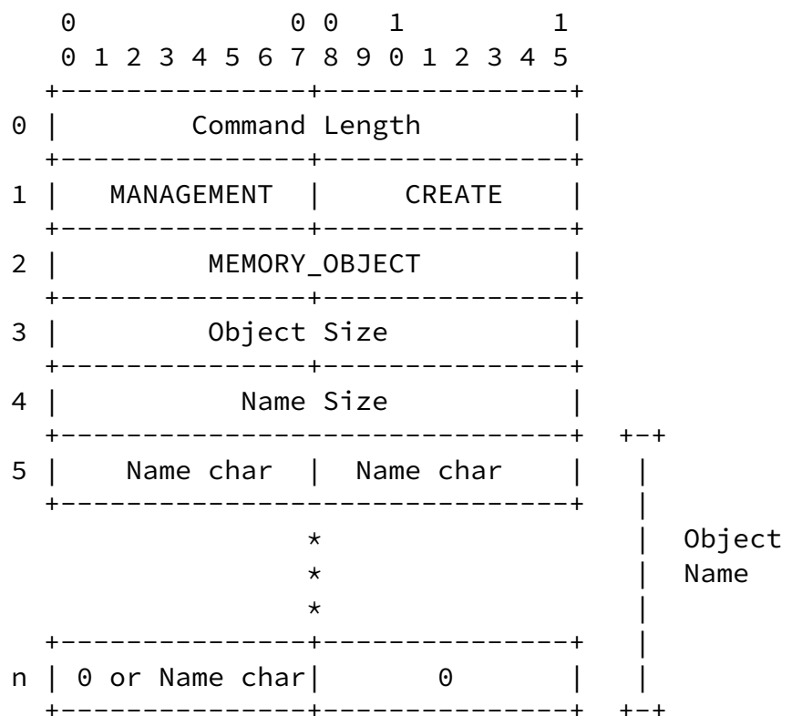
CREATE MEMORY_OBJECT Format Figure 45
