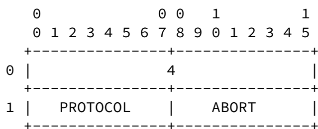
ABORT Command Format Figure 21
