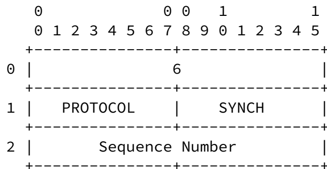
SYNCH Command Format Figure 19
