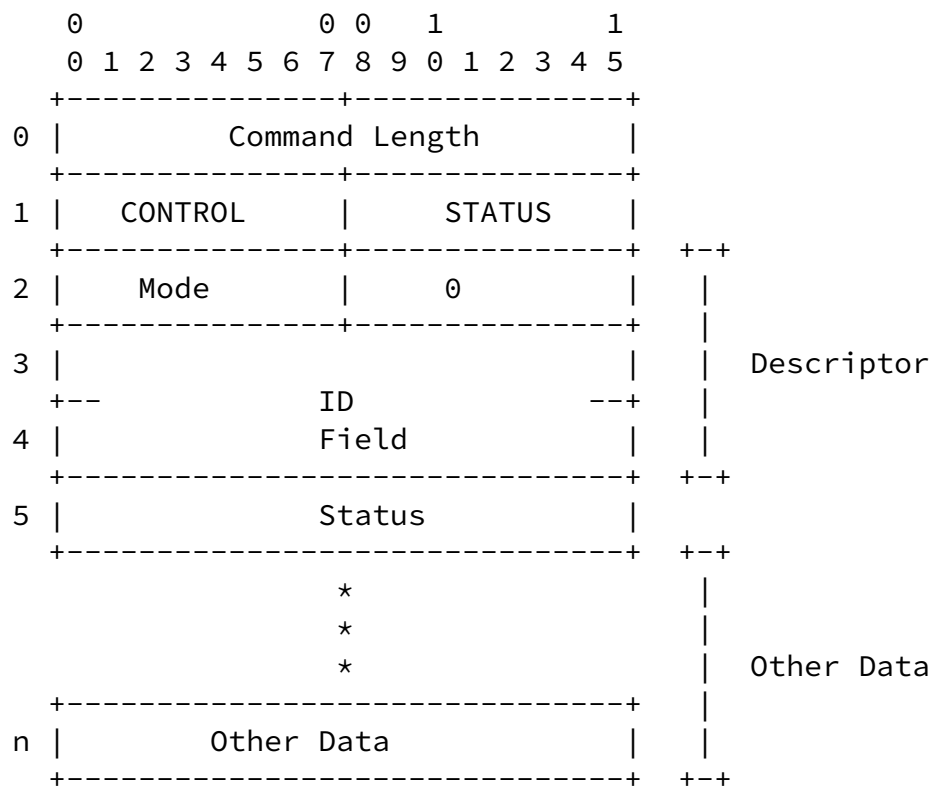
STATUS Reply Format Figure 40
