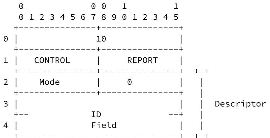
REPORT Command Format Figure 39
