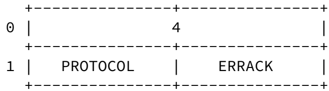
ERRACK Command Format Figure 25
