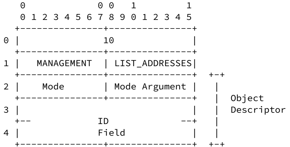
LIST_ADDRESSES Command Format Figure 49
