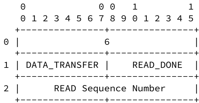
READ_DONE Reply Format Figure 29
