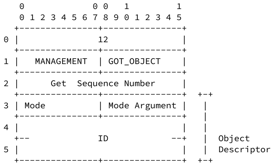
GOT_OBJECT Reply Format Figure 60
