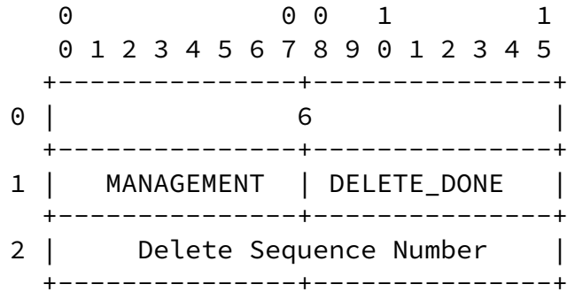
DELETE_DONE Reply Format Figure 48
