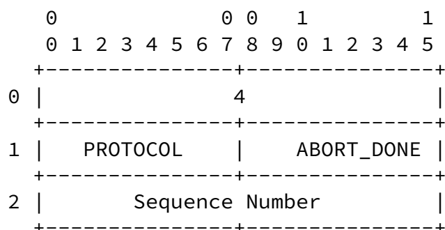
ABORT_DONE Reply Format Figure 22
