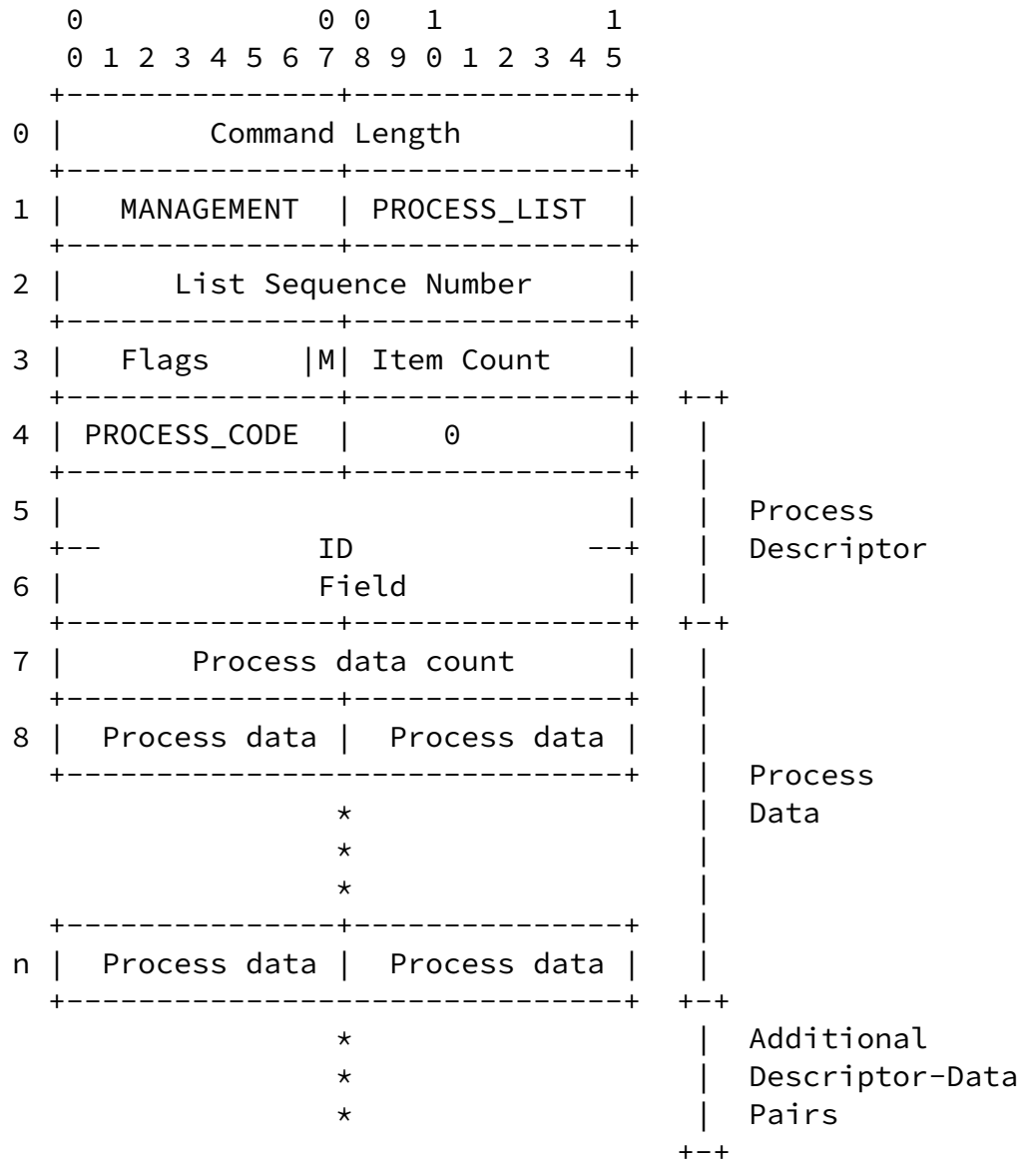
PROCESS_LIST Reply Format Figure 54
