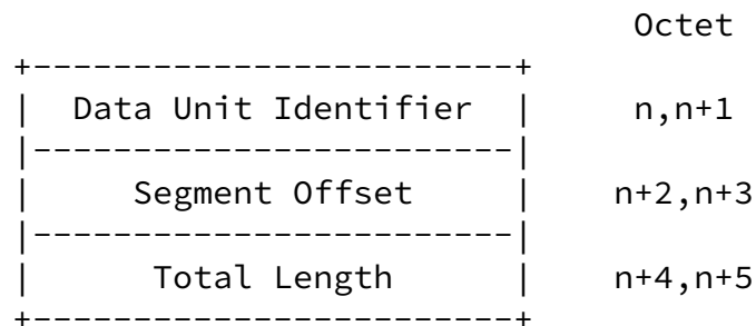
Figure 7-4. PDU Header--Segmentation Part
