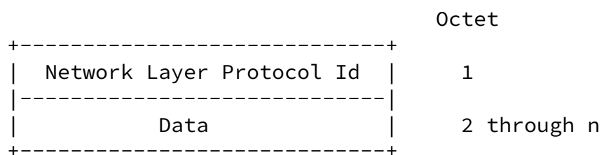
Figure 7-9. Inactive Network Layer Protocol
