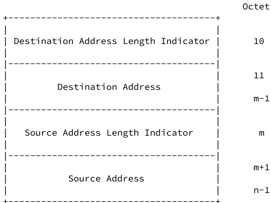
Figure 7-3. PDU header--Address Part
