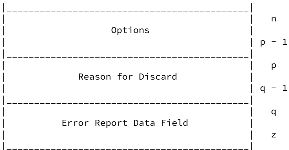
Figure 11: Error Report PDU
