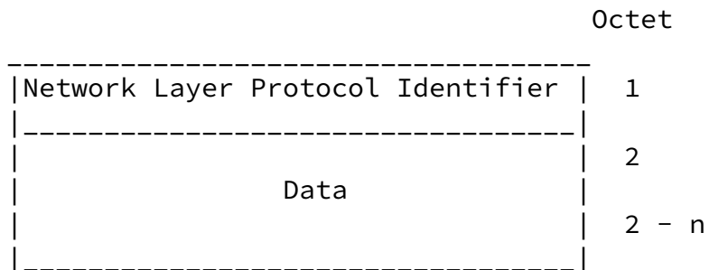
Figure 10: Inactive Network Layer Protocol
