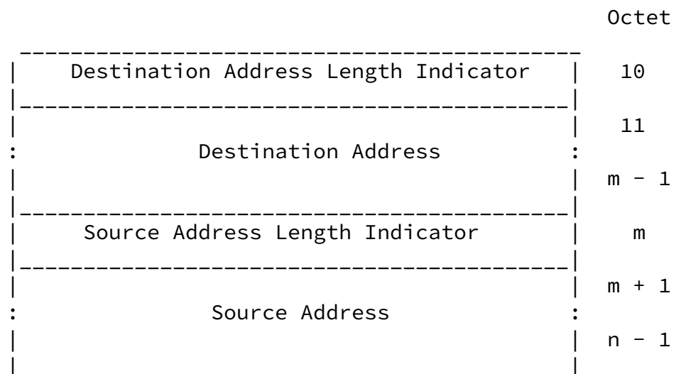
Figure 4: PDU Header -- Address Part
