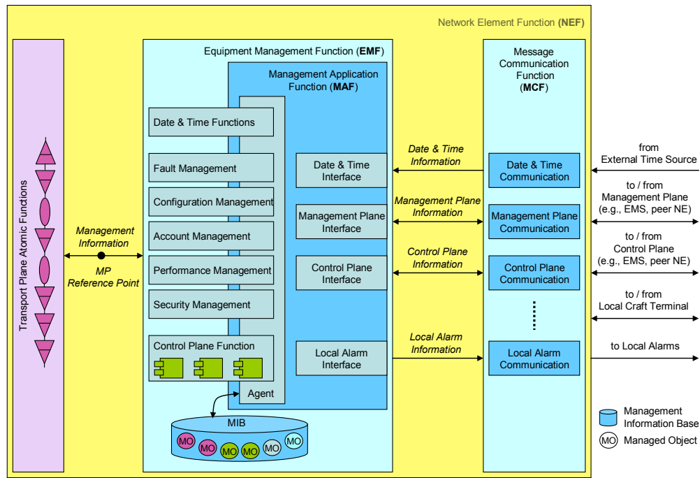
Figure 6.4/G.8151/Y.1374 — T-MPLS-TP Equipment Management Function
