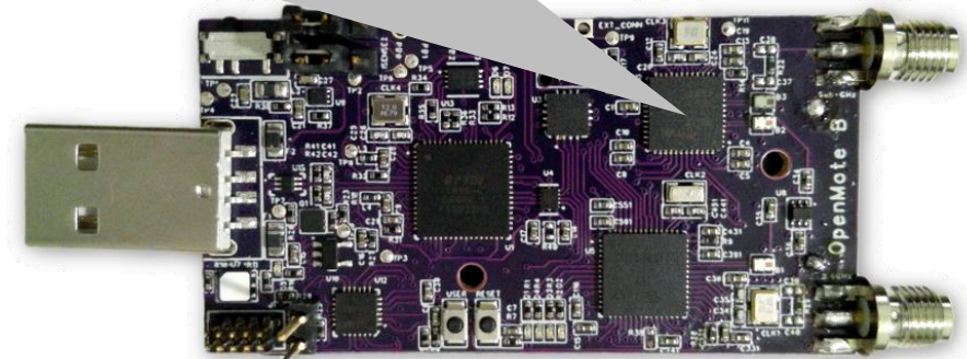
OpenMote B
