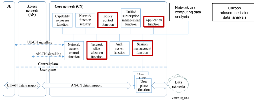
Potential enhancements toward network function of IMT-2020 network
