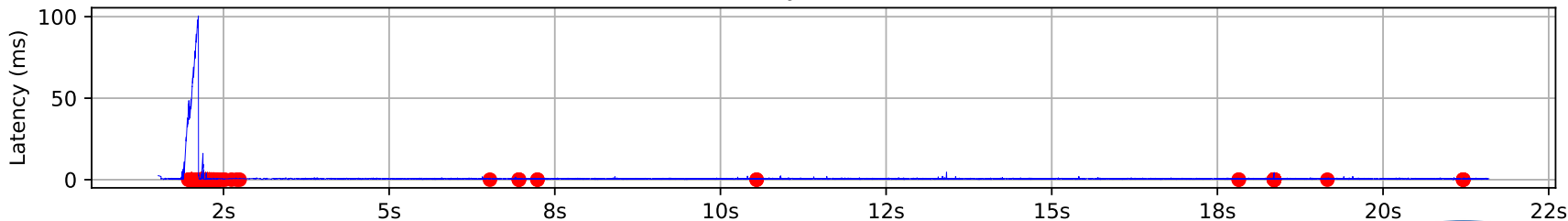
PDV Statistics
