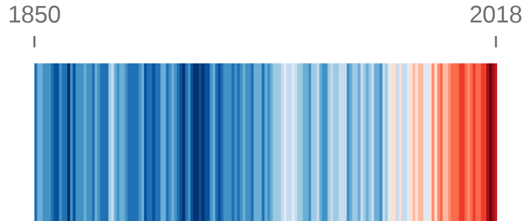
Climate stripes. Ed Hawkins, portrays the increase of average global temperature
