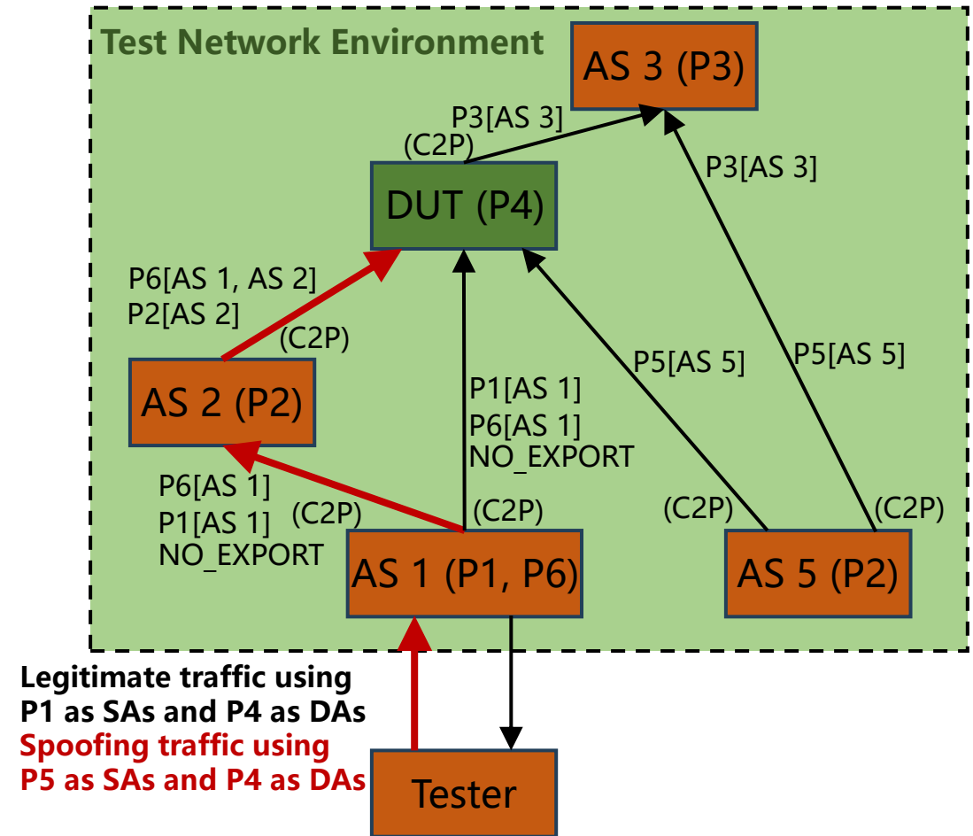
(a) Test Case 1: SAV for customer-facing ASes in inter-domain asymmetric routing scenario.
