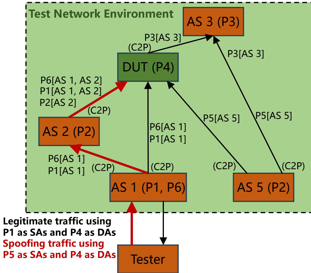
(a) Test Case 1: SAV for customer-facing ASes in inter-domain symmetric routing scenario.
