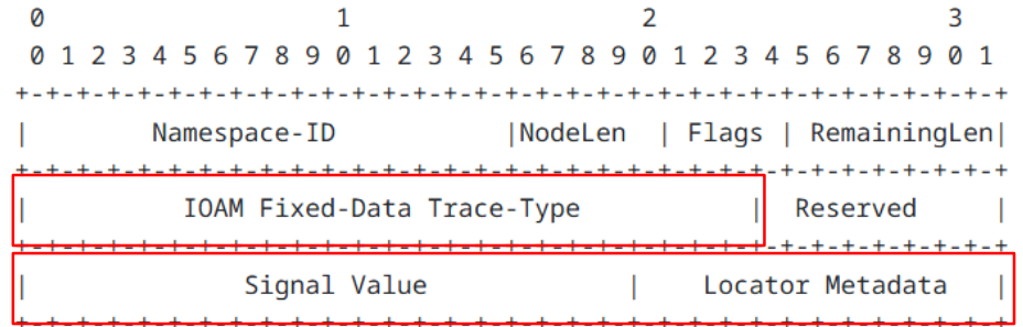
Figure 3: IOAM Trace Option carrying fixed-size aggregate data
