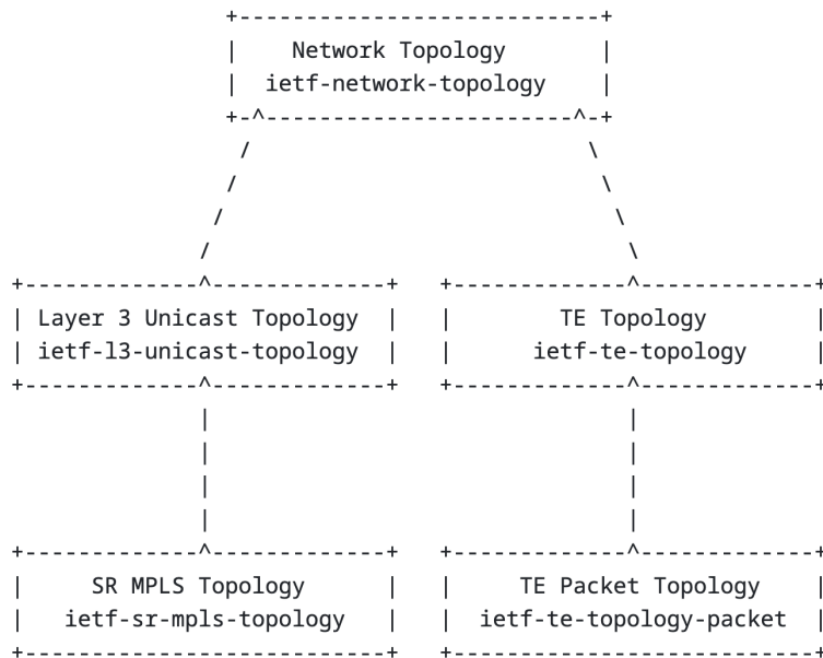
Figure: SR TE Topology Instance Inheritance Relations
