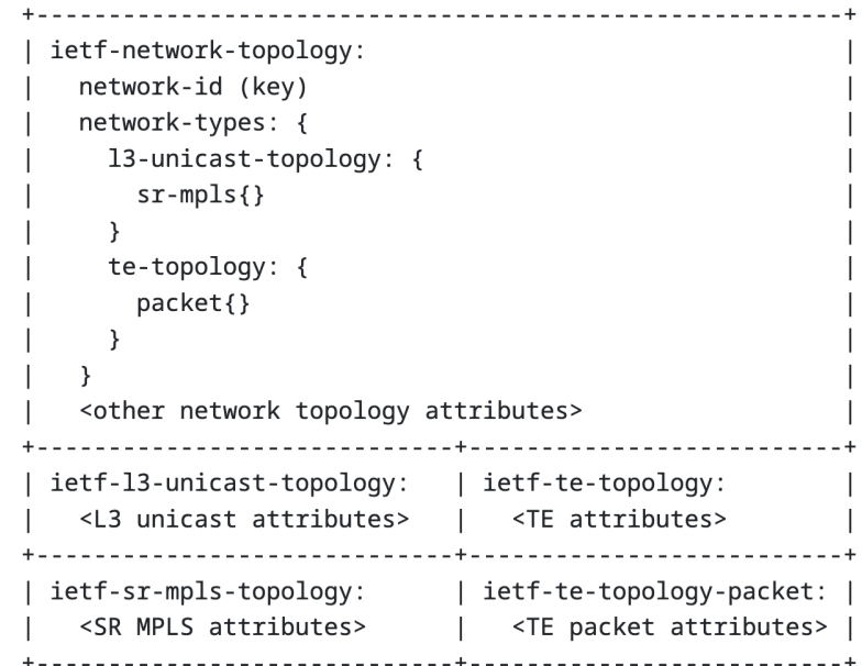
Figure: SR TE topology instance data structure
