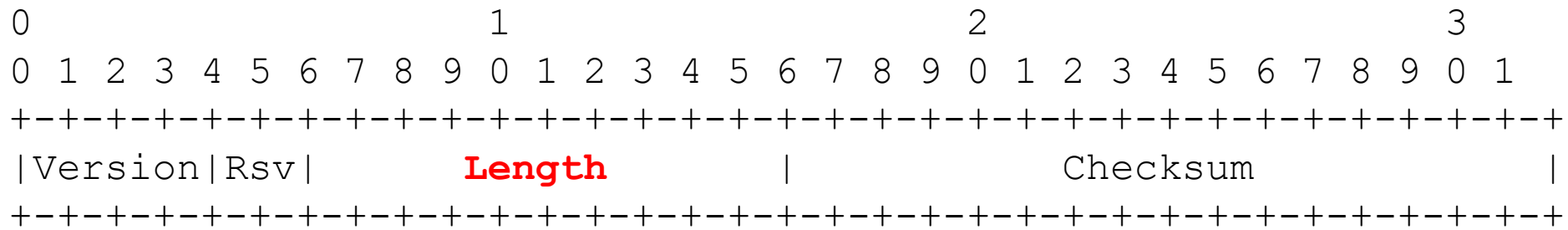
ICMP Extension Header With Length Field
