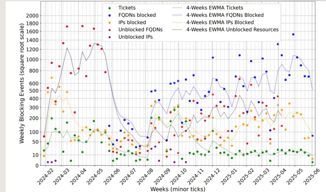
Fig. 1: Weekly blocking and unblocking events with 4-weeks Exponentially Weighted Moving Average (square-root scale)
