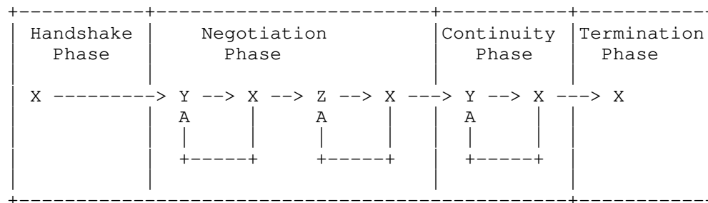
Figure 16 Phases & client behaviors.
