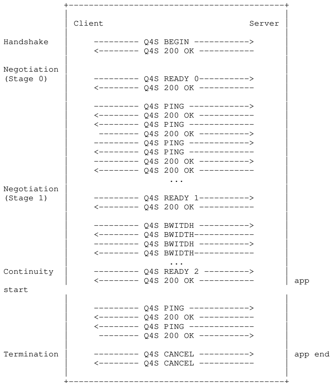
Figure 2 Successful Q4S message exchange.
