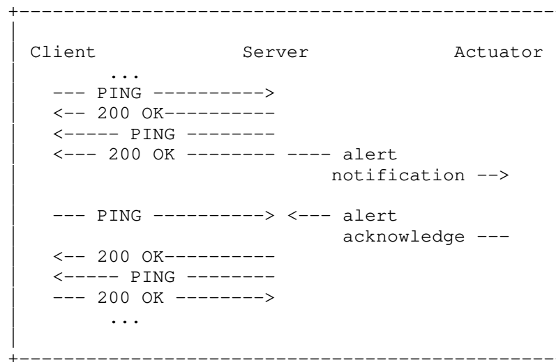
Figure 13 Continuity in Reactive alerting mode
