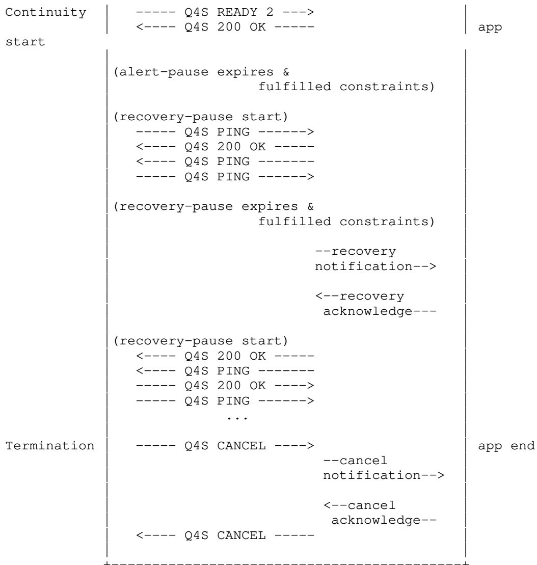
Figure 4 Reactive alerting mode.
