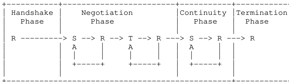
Figure 17 Phases & server behaviours.
