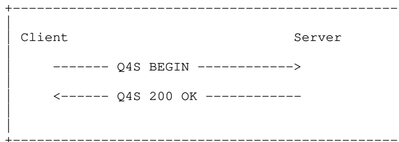
Figure 7 Handshake phase.
