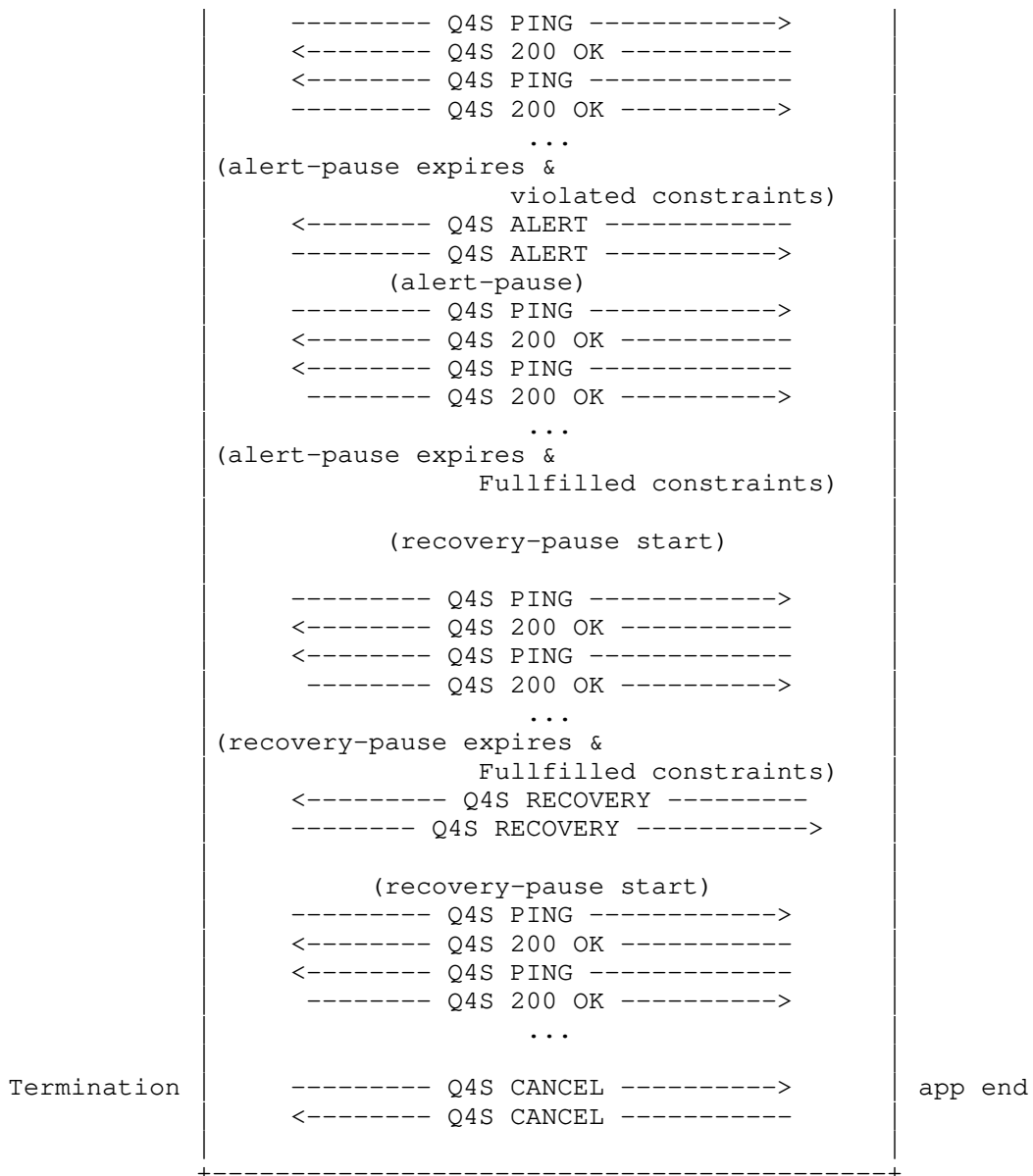
Figure 3 Q4S-aware-network alerting mode.
