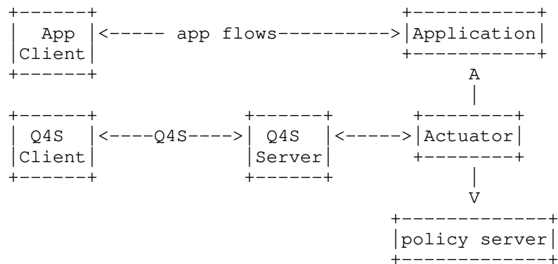
Figure 1 Reactive scenario
