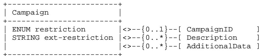
Figure 8: Campaign Class
