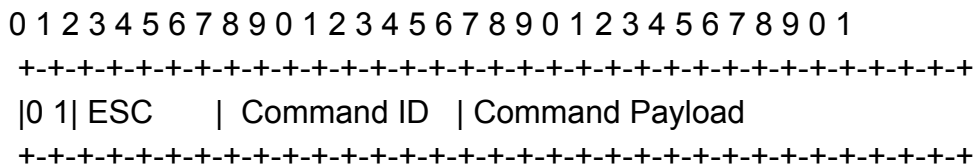
G.9903 Frame Format with ESC Byte ( draft-chairs-6lo-dispatch-iana-registry-00 )
