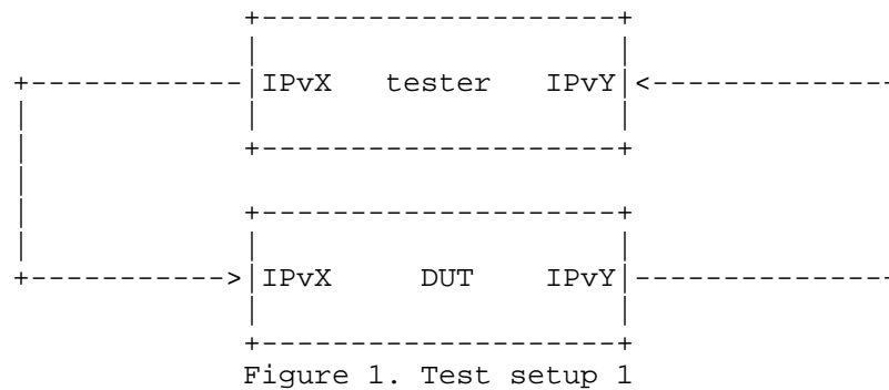
Figure 1. Test setup 1
