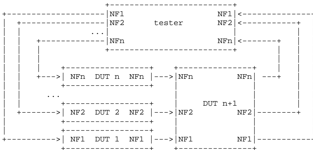
Figure 4. Test setup 4
