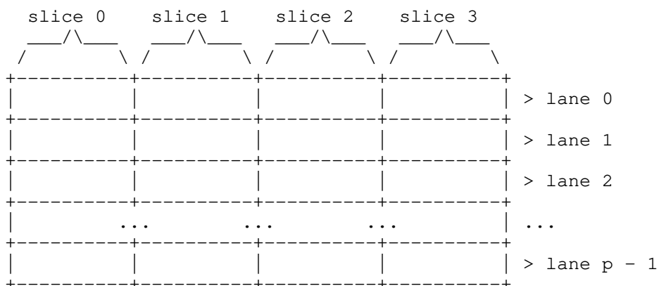
Single-pass Argon2 with p lanes and 4 slices
