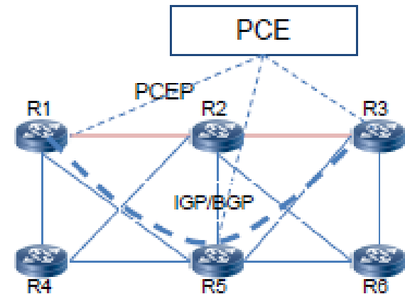
PCE in Native IP Network
