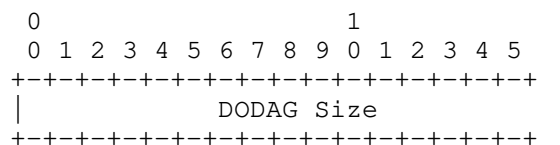
Figure 2: DODAG Size field Format
