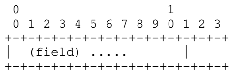
Figure 1: DODAG Size Object Body Format
